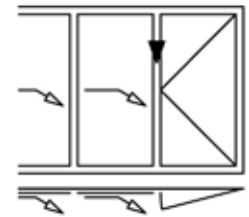
Detail 35HSW-11-6
