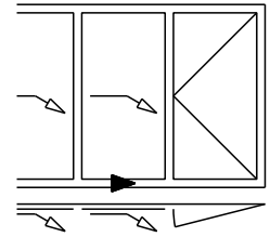
Detail 35HSW-2-2
