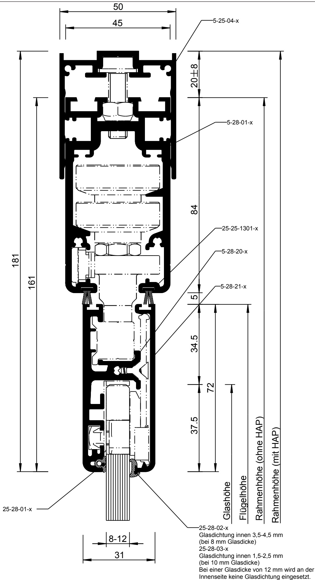
Detail 25 XXL-1-7
