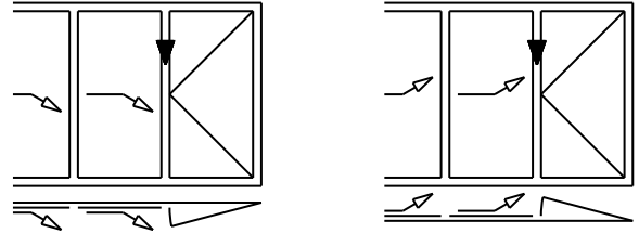
Detail 25 XXL-11-4
