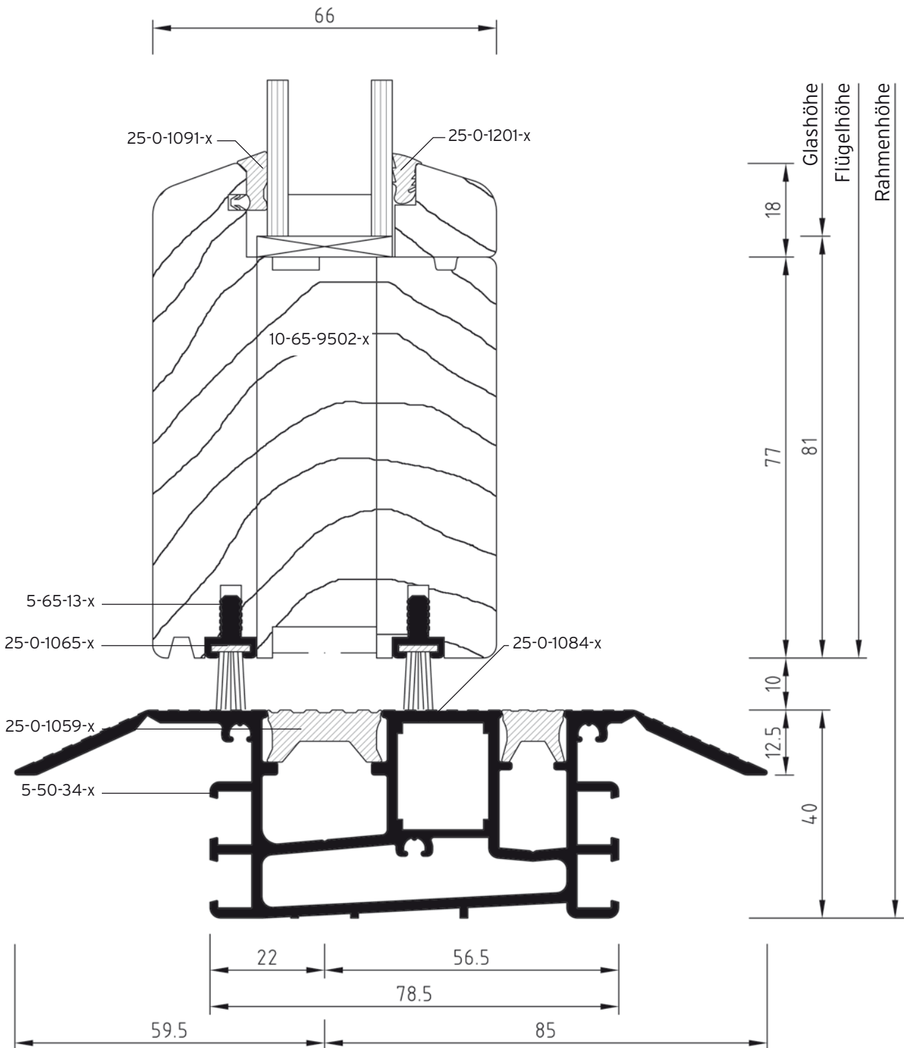
Detail 65HSW-2-12
