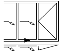
Detail 65HSW-2-4
