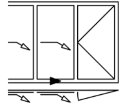
Detail 65HSW-2-6
